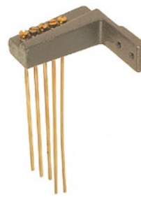
CO447.5E * Longest rod - 6" * Shortest rod - 4-1/2"
